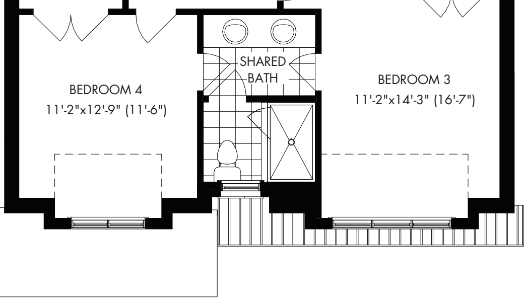
PARTIAL SECOND FLOOR ELEV. C
