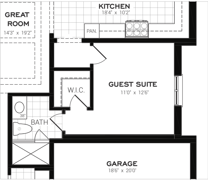
OPTIONAL GROUND FLOOR WITH GUEST SUITE
