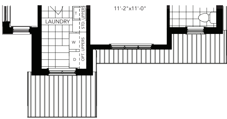
PARTIAL SECOND FLOOR ELEV. C
